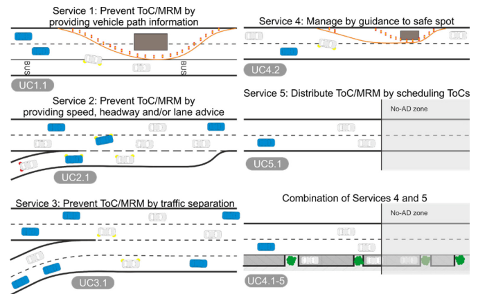
Fig. 1. Excerpt of investigated TransAID services and use cases. Blue vehicles are CAVs.
