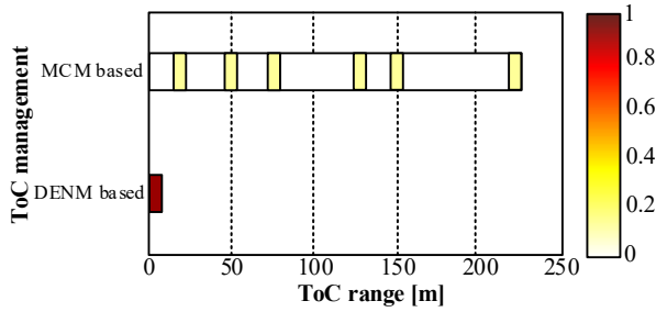
Fig. 8. ToC distribution
