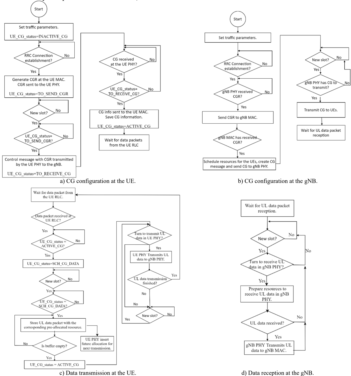
Fig. 2. Operation of the CG scheduling at the UE and gNB.
